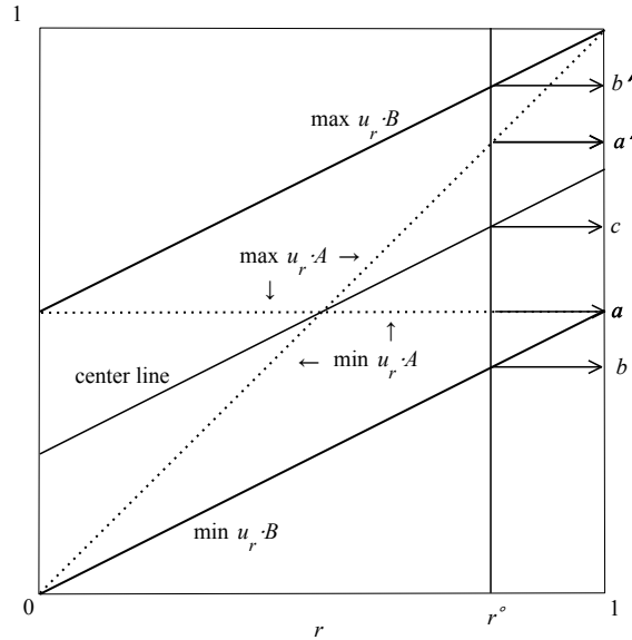
Figure 5(b) [a, a'] = [\min u_{r^o} \cdot A, \max u_{r^o} \cdot A] [b, b'] = [\min u_{r^o} \cdot B, \max u_{r^o} \cdot B] c = \frac{1}{2}a + \frac{1}{2}a' = \frac{1}{2}b + \frac{1}{2}b'
