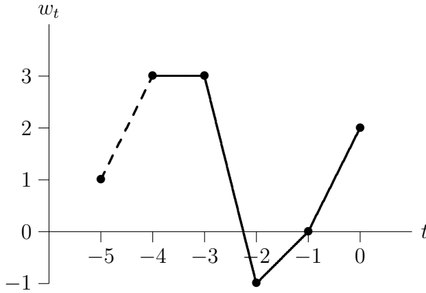
Figure 2: Difference monotonicity.
