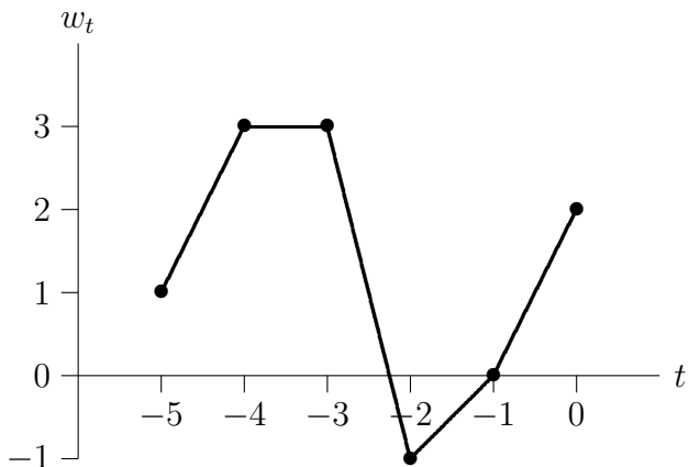
Figure 1: The wealth stream w = (1, 3, 3, -1, 0, 2) .
