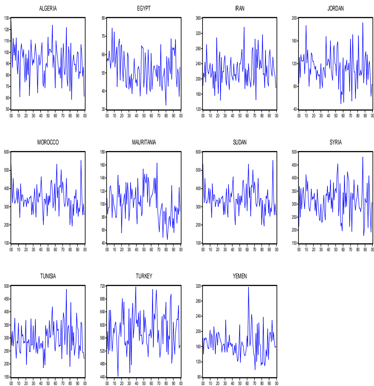
Figure A1: Average annual precipitation by country, mm per year (1900–2000)
