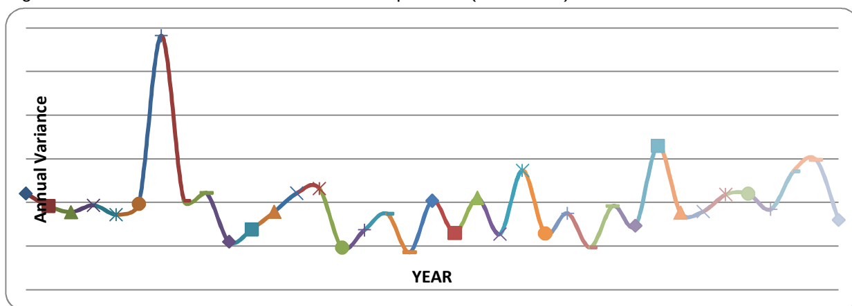
Figure 4a: Trends in the variance of coastal temperature (1972-2008)
