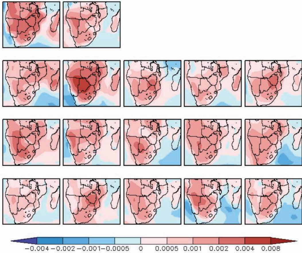
Figure 9: Maps of the transformation coefficients, dC_{x,y}/dT_{Global} (units of K^{-1} ) over the southern Africa for surface air temperature. Shown are the results for each model of the IPCC AR4 collection of the seasonally averaged pattern shifts averaged for December-February.
