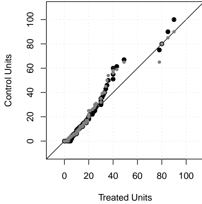
Figure 3: QQ Plot of Covariate HLEDU (Treated versus Raw and Matched)
