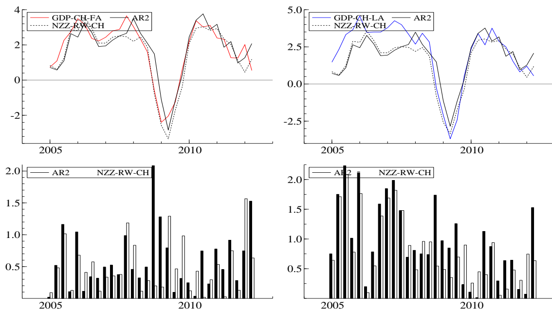
Figure 5: Quarterly year-on-year real GDP growth: Forecasts and absolute forecast errors from AR(2) and ARDL(2,0)-NZZ-RW-CH models
