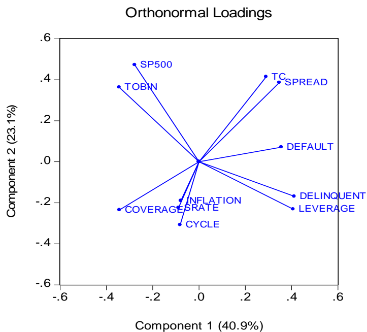
Fig. 2. Eigen vector loadings (1 and 2)
