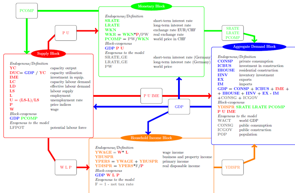
Figure 1: The KOF macroeconomic model
