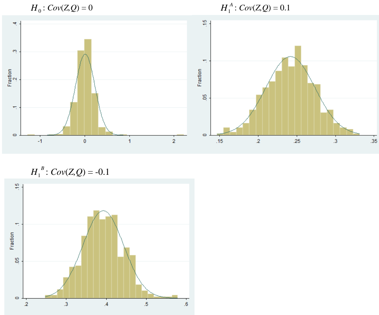
Figure 3. Empirical distribution of the test statistic under the null and two simulated deviations from the null hypothesis Cov(Z,Q) = 0 . Simulated data with a sample size of 5000 observations and 500 replications
