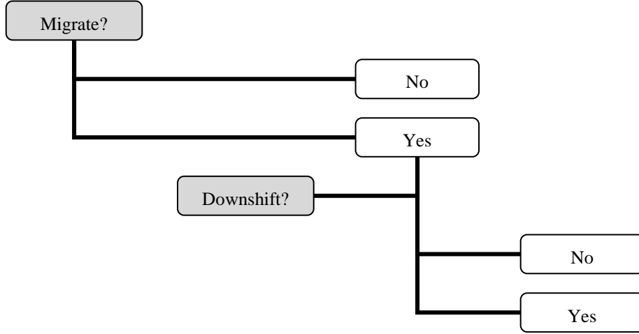
Figure 1: Decision tree
