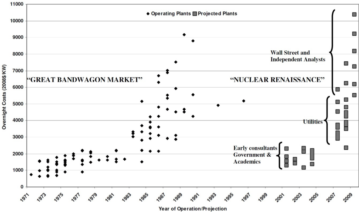
Figure 4: Evolution of cost estimates for nuclear power plants.
