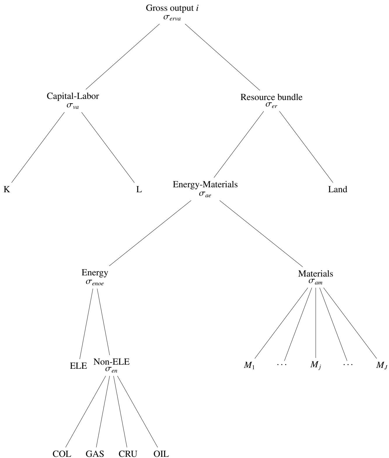
Figure A.11: Structure of production for i \in \{AGR\} .
