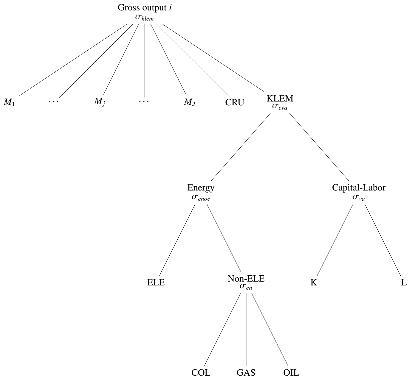
Figure A.13: Structure of production for i \in \{\text{OIL}\} .
