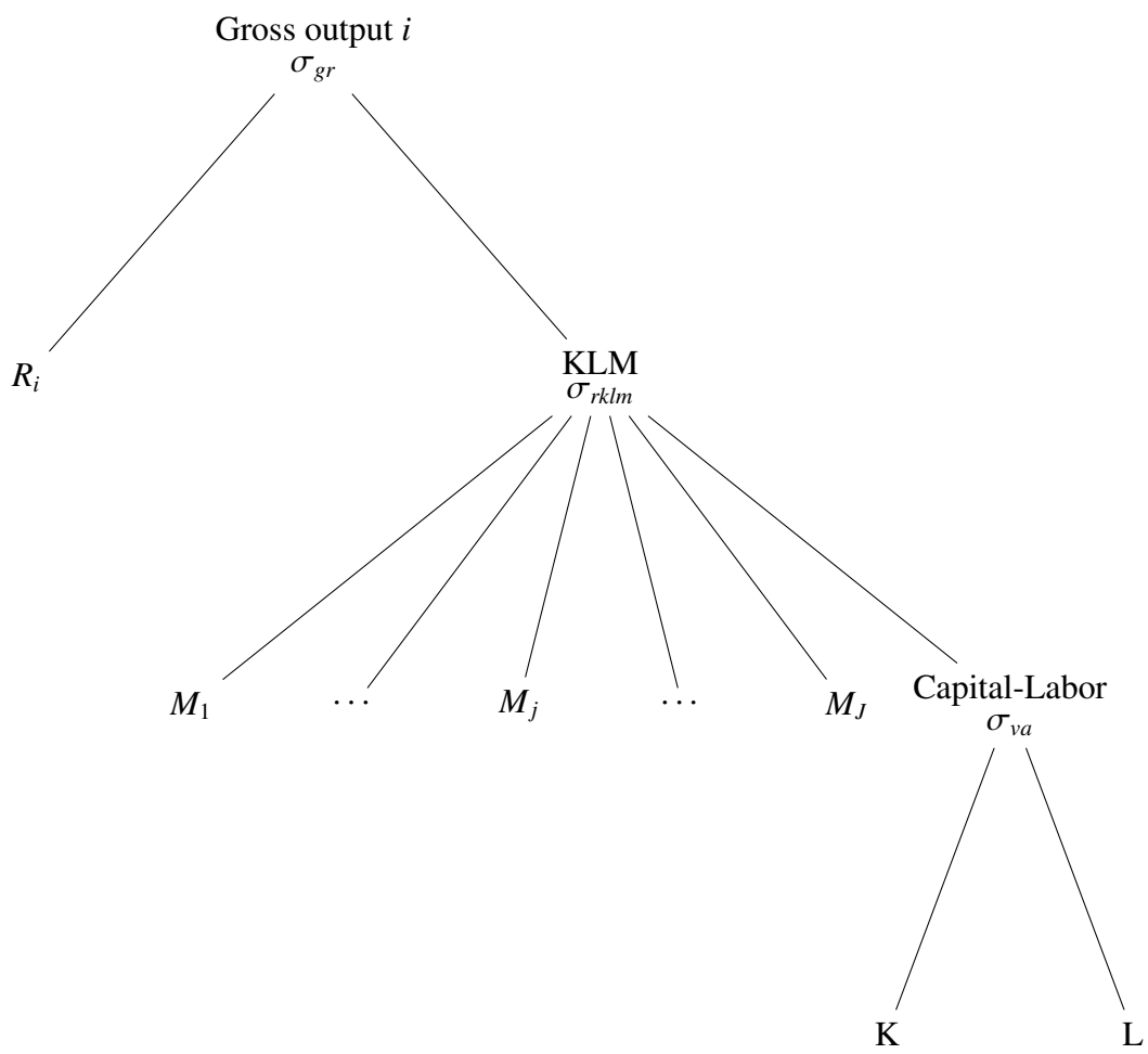
Figure A.12: Structure of primary energy sectors i \in \{\text{COL, CRU, GAS}\} .
