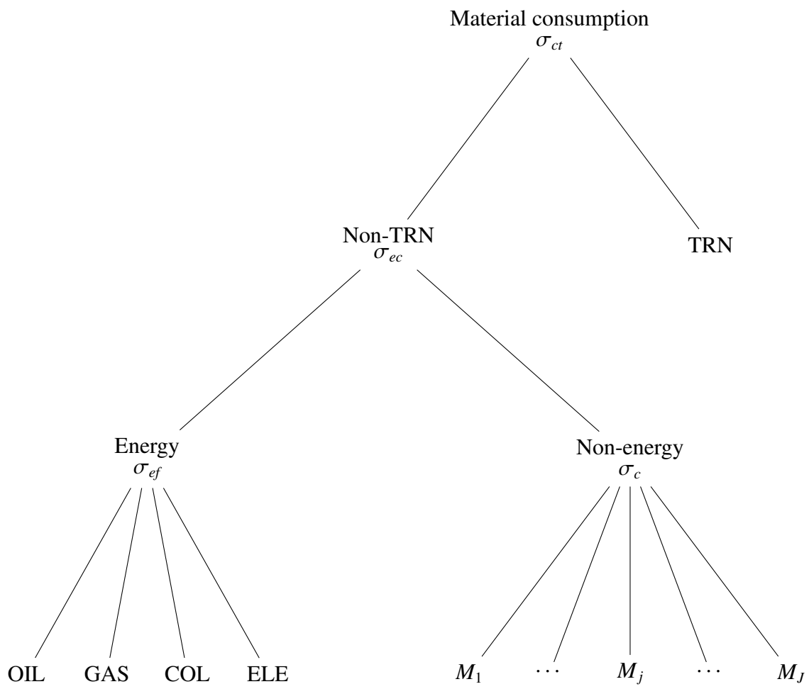
Figure A.15: Structure of private material consumption.
