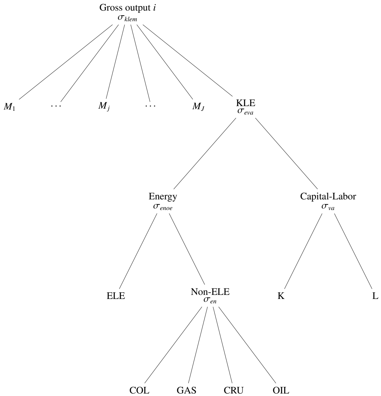
Figure A.10: Structure of production for i \in \{TRN, EIS, SRV, CRP, I, S, NFM, NMM, PPP, MAN\} .
