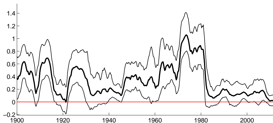
Figure 17: \hat{b}_f : Median and 68% central posterior bands for the time-varying regression coefficient inflation on primary deficits over debt. Robustness check with 3m real interest rates instead of 6m interest rates.
