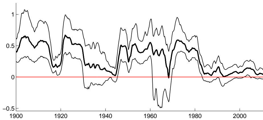
Figure 18: \hat{b}_f : Median and 68% central posterior bands for the time-varying regression coefficient inflation on primary deficits over debt. Robustness check with real debt growth instead of primary deficits over debt.
