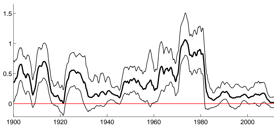
Figure 16: \hat{b}_f : Median and 68% central posterior bands for the time-varying regression coefficient inflation on primary deficits over debt. Robustness check with 3m nominal interest rates instead of 6m interest rates.
