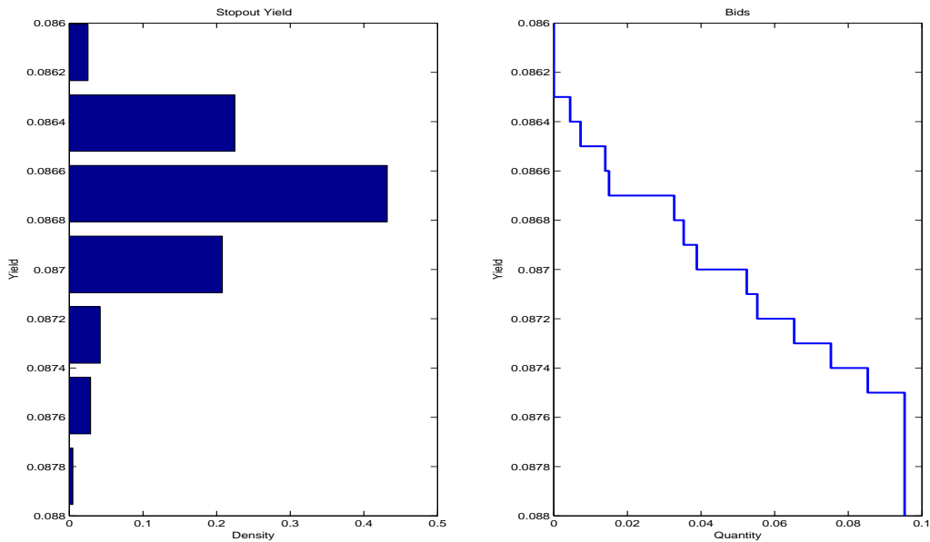
Figure 4.2: Stopout Yields
