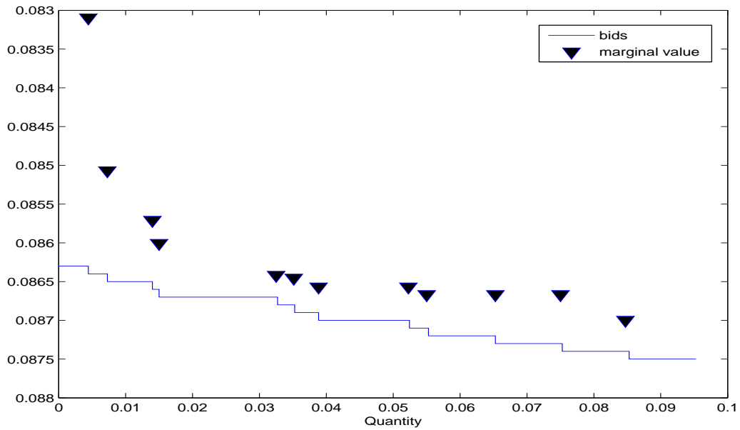
Figure 4.4: Bidder valuations
