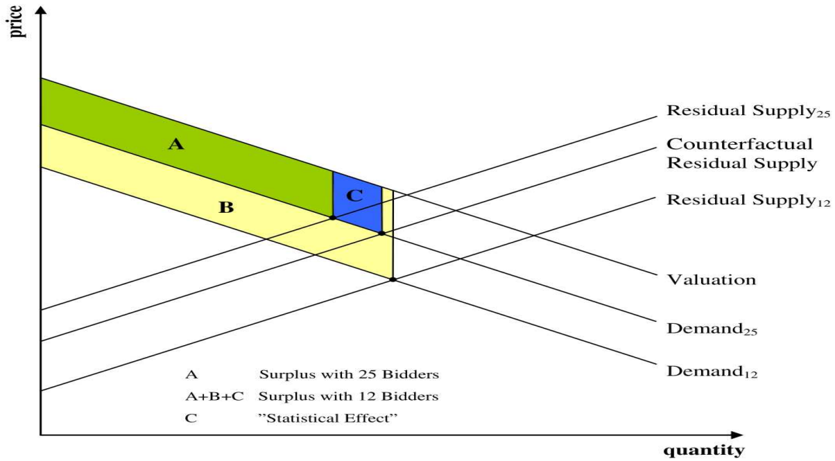
Figure 4.6: Statistical effect
