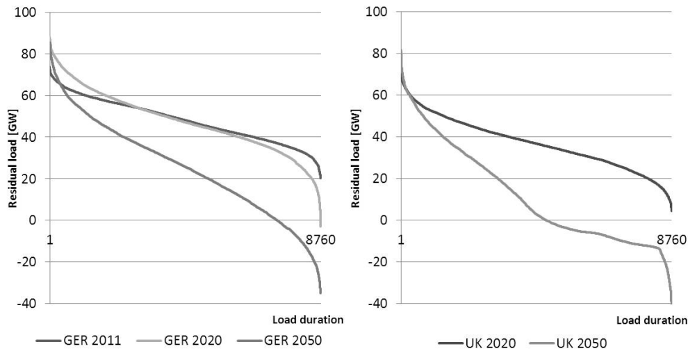
Figure 1: Residual load duration curve for Germany(left) and UK (right) [GW]
