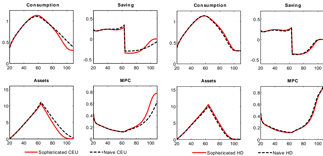
Figure 7: Life-cycle profiles of the naive and sophisticated CEU agent (a) CEU Agent (b) HD Agent
