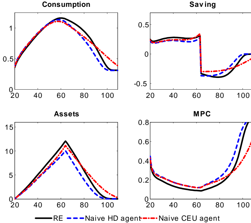
Figure 13: Life-Cycle Profiles of Naive CEU and HD Agents compared to RE
