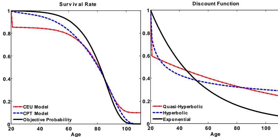
Figure 2: Survival Rates and Discount Functions
