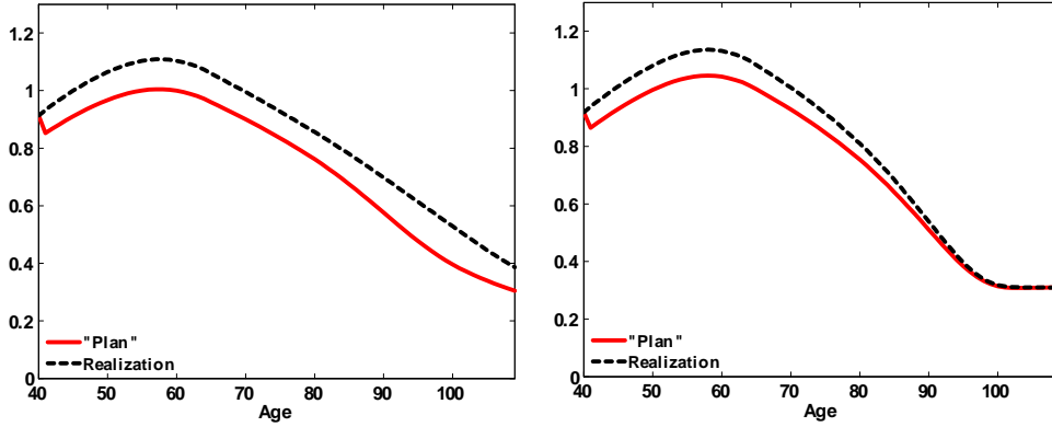
Figure 12: Planned and Realized Consumption at Planning Age 40 (a) Naive CEU (b) Naive HD
