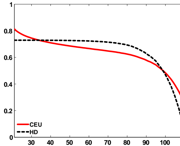
Figure 8: Effective Discount Factors from age h to age h+1
