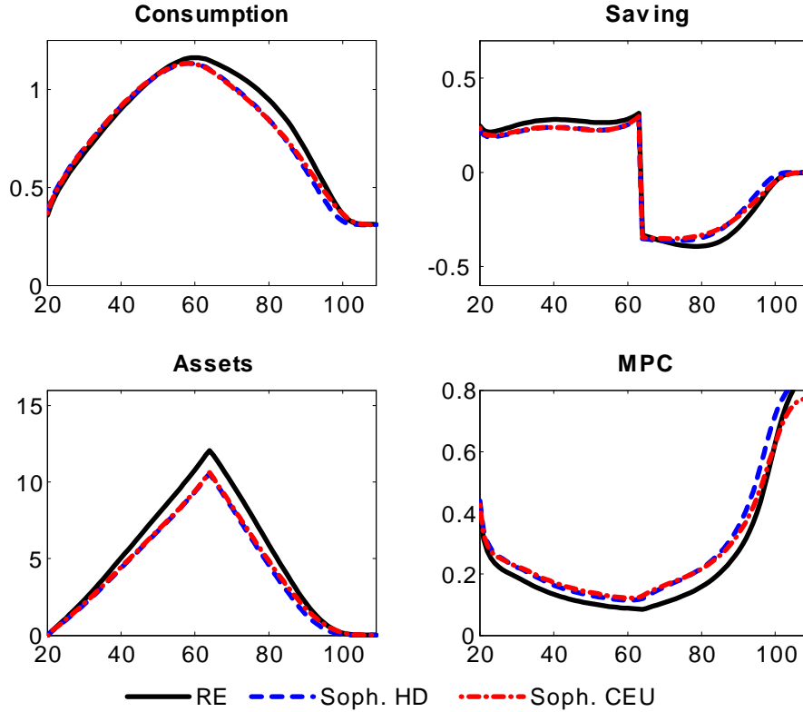
Figure 14: Life-Cycle Profiles of Sophisticated CEU and HD Agents compared to RE
