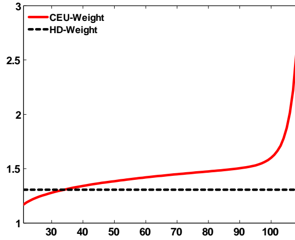
Figure 9: Weights in the Generalized Euler-Equation of Sophisticated Agents
