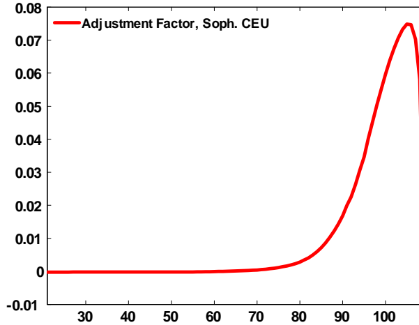
Figure 10: Adjustment Factor for the Sophisticated CEU Agents
