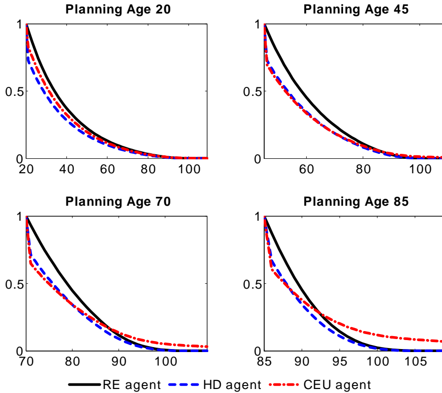
Figure 5: Effective discount functions
