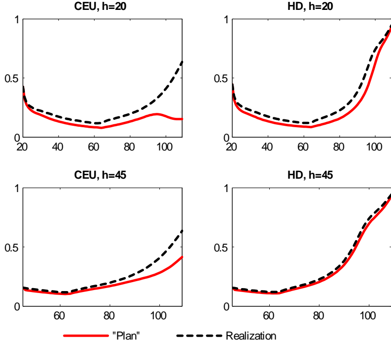
Figure 11: Planned and realized MPC for CEU and HD agents
