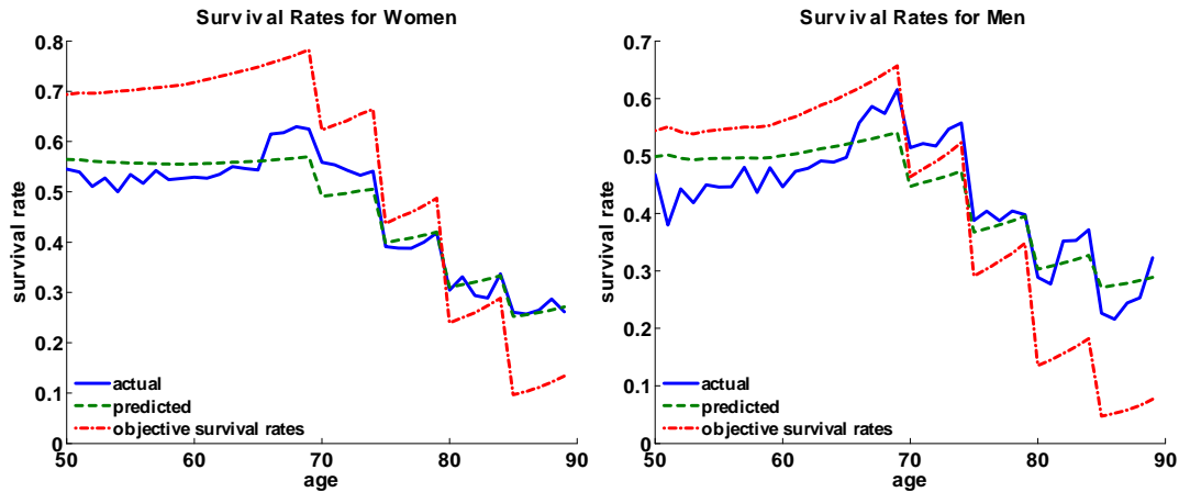
Figure 3: Objective, subjective and predicted survival rates
