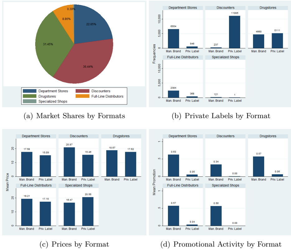
Figure 1: Descriptive Statistics
