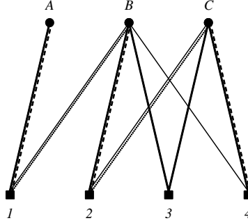
Figure 4: Symmetric difference operation ( N \Delta M )
