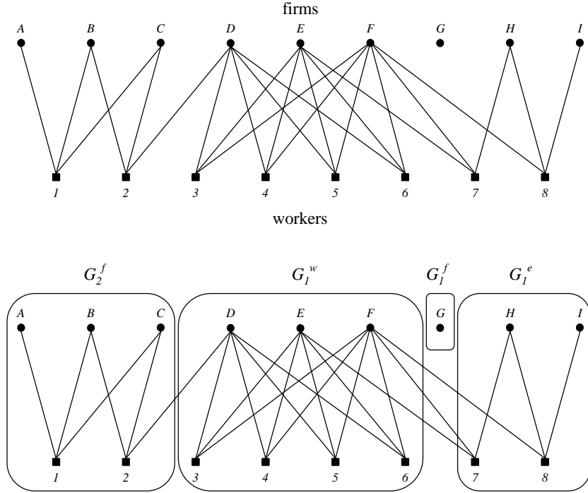
Figure 2: Graph-Decomposition
