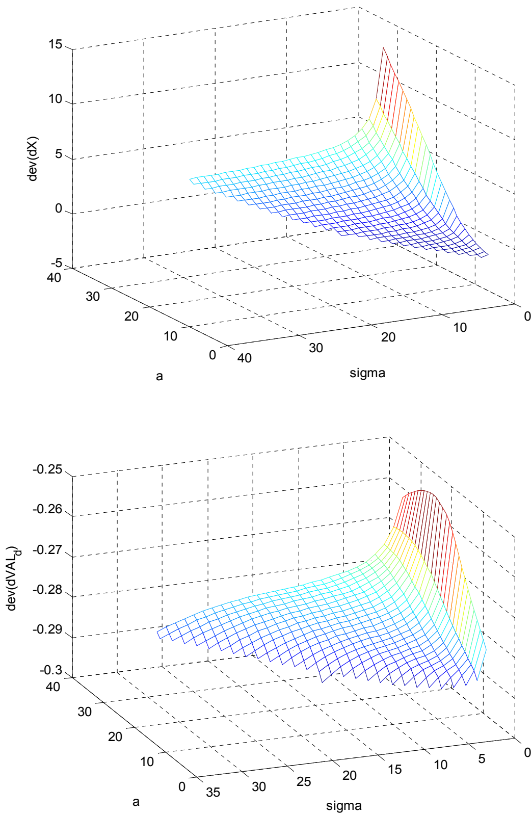
Figure 3: Moment Deviations as a Function of a_\gamma and \sigma (trade and productivity growth, first moment; alternative modeling of tariffs)
