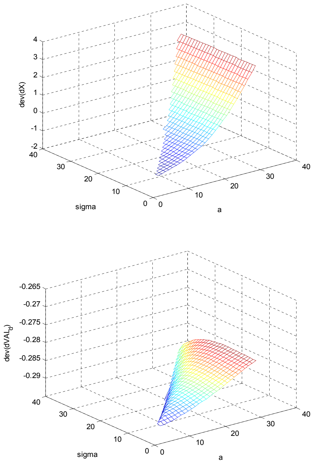
Figure 2: Moment Deviations as a Function of a_\gamma and \sigma (trade and productivity growth, first moment; baseline model)
