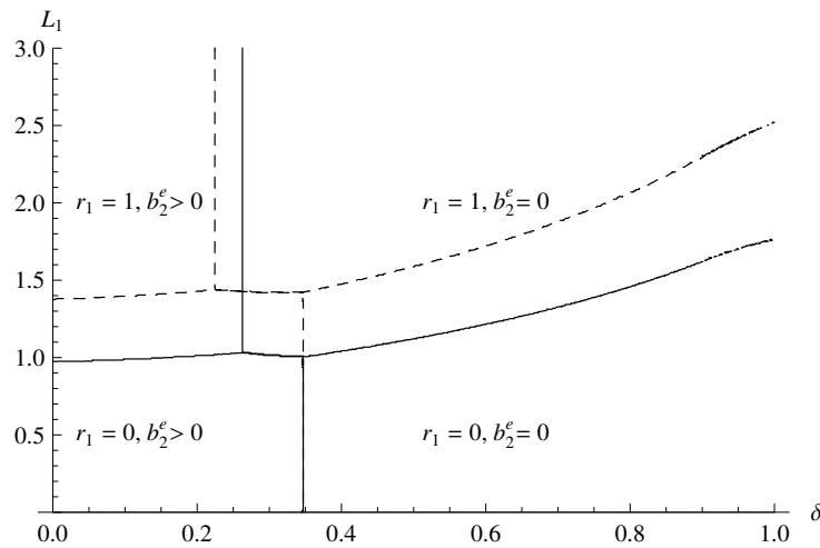
Figure 4: Default and official lending regions for b_{02} = 2 (solid) and b_{02} = 3 (dashed).
