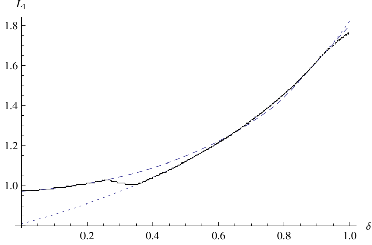
Figure 3: \hat{L}_1^{\text{PR}} (dotted), \hat{L}_1^{\text{OF}} (dashed), \hat{L}_1 (solid) as functions of \delta .
