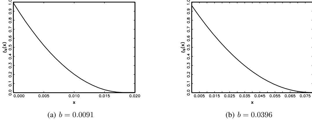
Figure 2: \xi_b(x)
