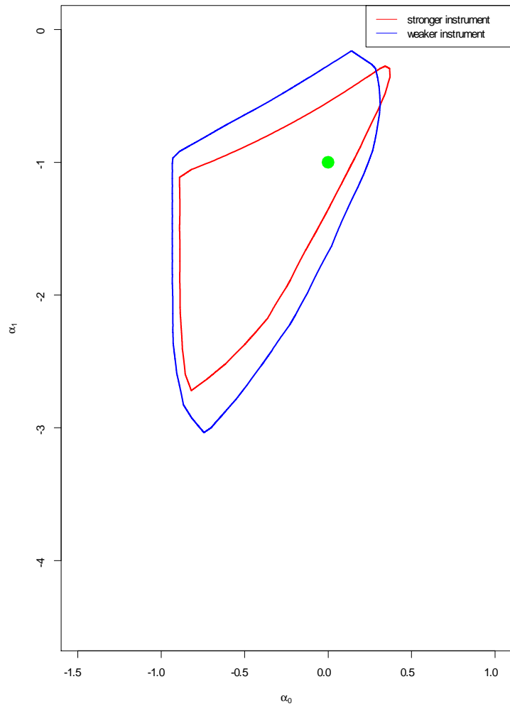
Figure 1: Projections of identified sets for (\alpha_0, \alpha_1) using weaker and stronger instruments for a process in which X is endogenous. The illustration is computed as described in Appendix B, with alphahull parameter set to 5.
