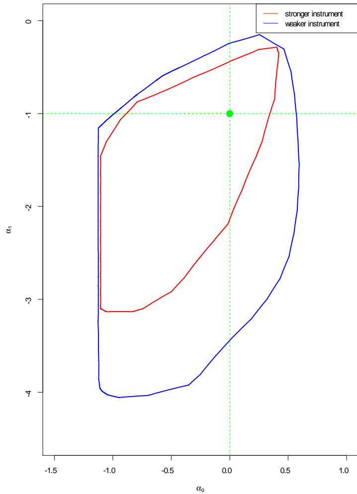
Figure 2: Projections of identified sets for (\alpha_0, \alpha_1) using weaker and stronger instruments for a process in which X is exogenous. The illustration is computed as described in Appendix B, with alphahull parameter set to 5.
