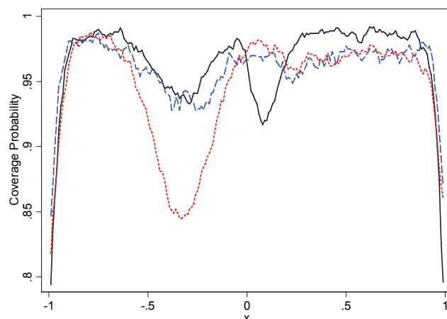
(b) g(x) = \sin(3\pi x/2)/\{1 + 18x^2[\text{sgn}(x) + 1]\} .
