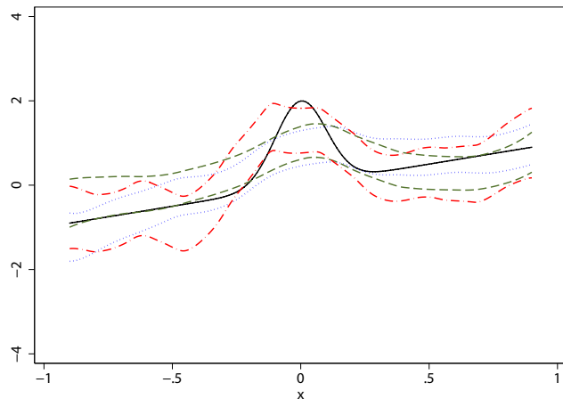
(c) Conventional method with explicit bias correction: \lambda = 0.05
