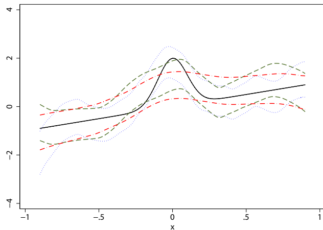
(a) Proposed new method: 0.90 quantile.
