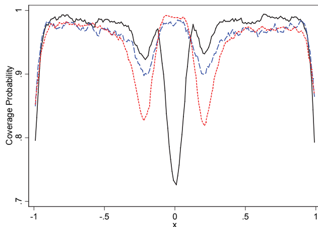
(a) g(x) = x + 5\phi(10x) .
