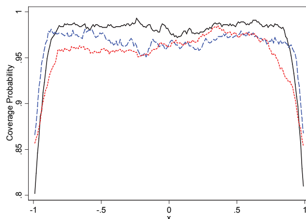
(c) g(x) = \sin(\pi x/2)/\{1 + 2x^2[\text{sgn}(x) + 1]\}
