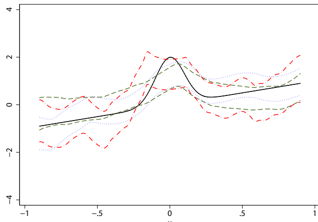
(b) Conventional method with undersmoothing: \gamma = 0.7
