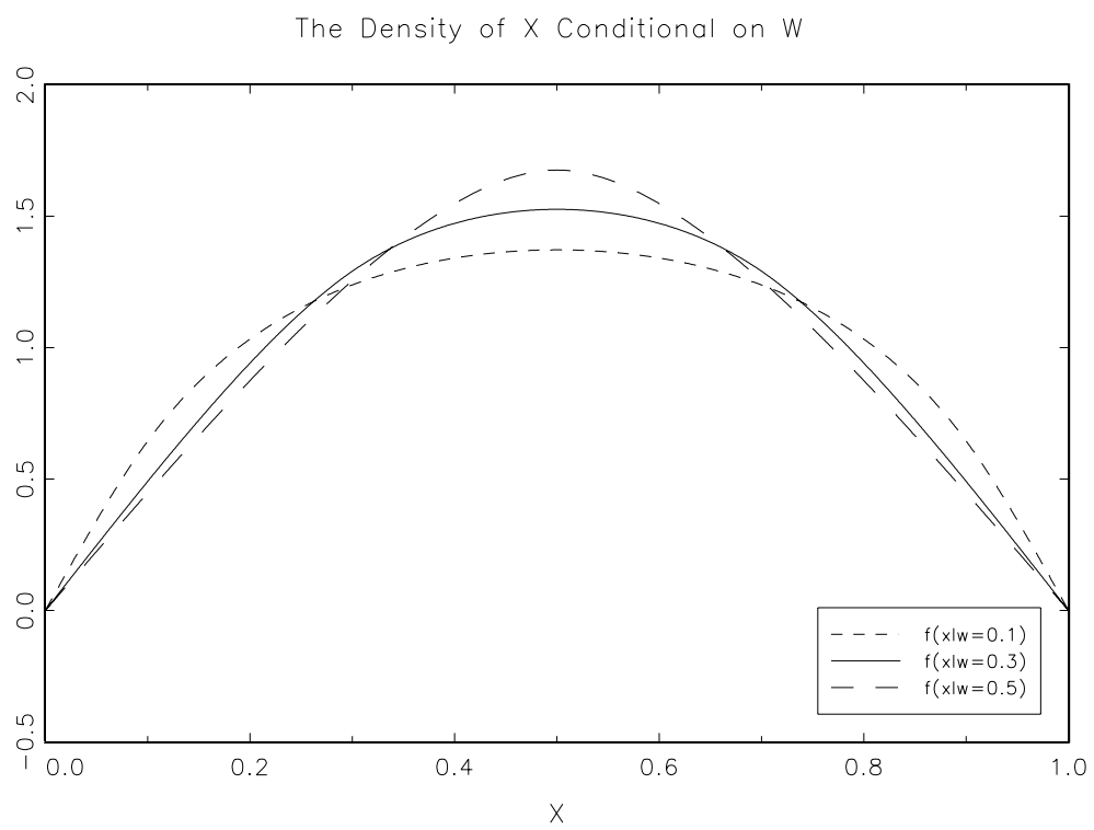
Figure 2: The Density of X Conditional on W
