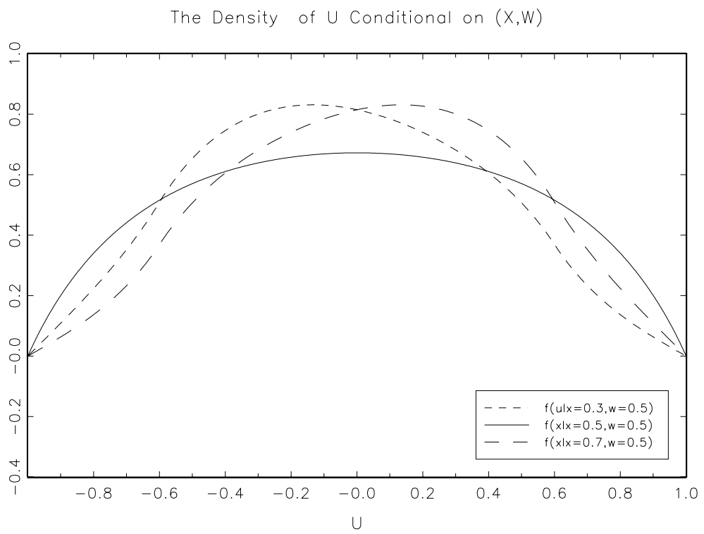
Figure 3: The Density of U Conditional on X and W
