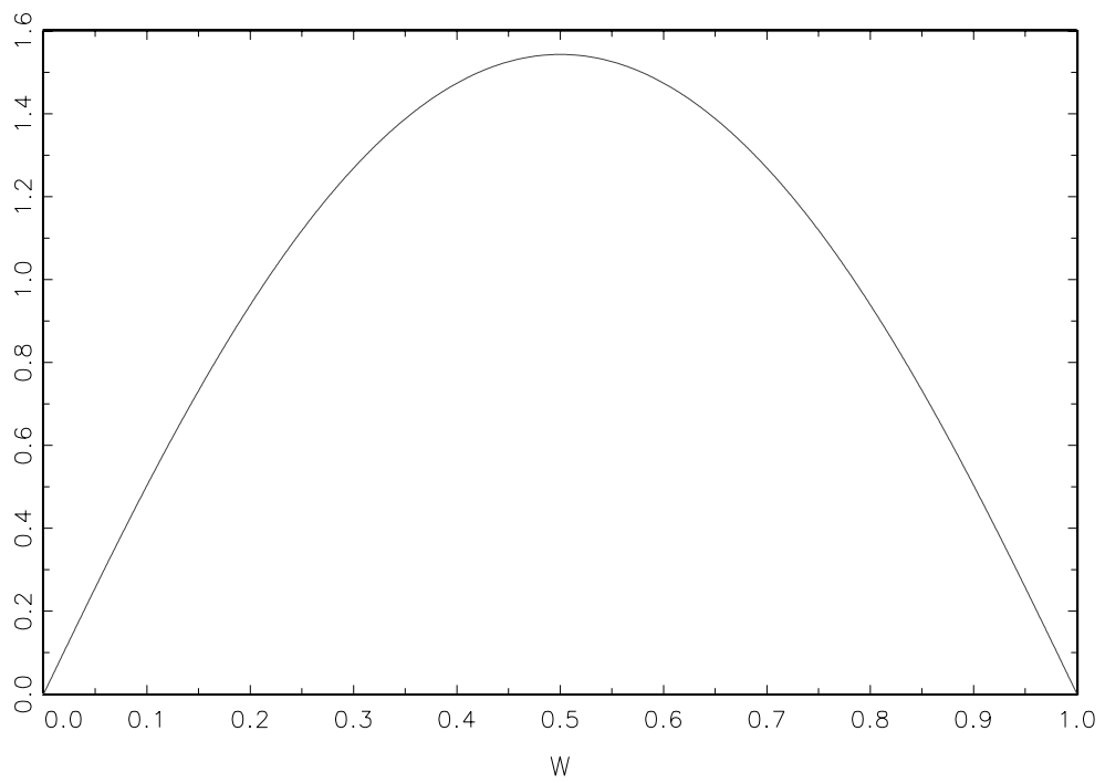
Figure 1: The Density of W
