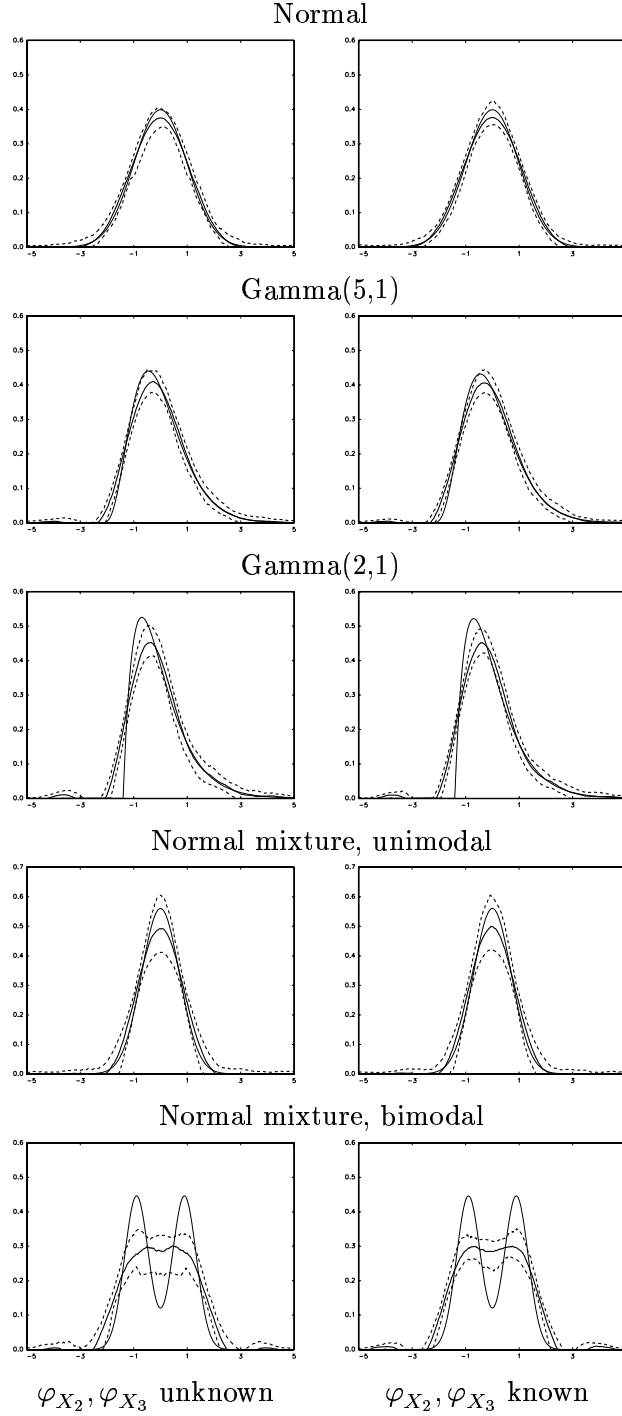
Figure 3: Monte Carlo estimates of f_{X_1} in the measurement error model (16) with normal errors, using a fourth-order kernel
