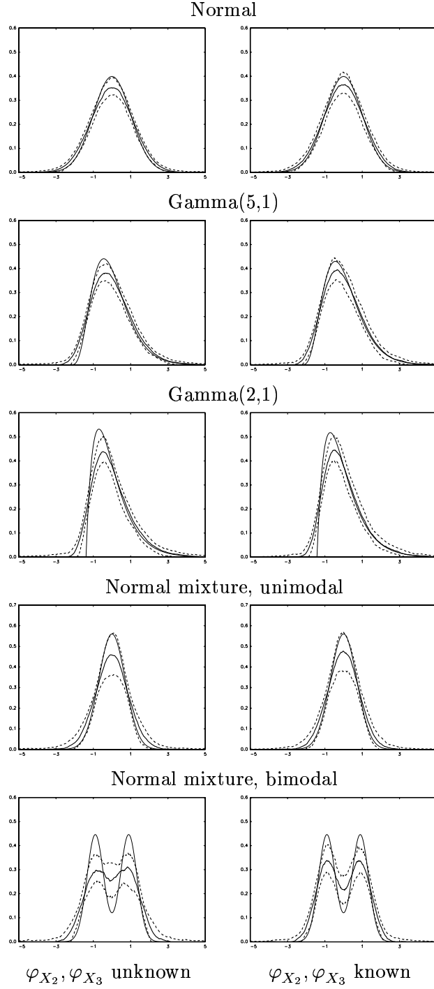
Figure 2: Monte Carlo estimates of f_{X_1} in the measurement error model (16) with Laplace errors
