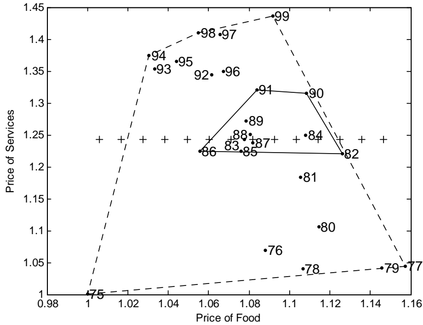
Figure 3: Relative prices, 1975 – 1999.
