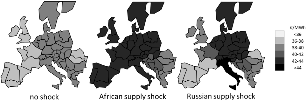
Figure 6: Electricity prices in dependence of gas supply shock in 2030, 80%GREEN
