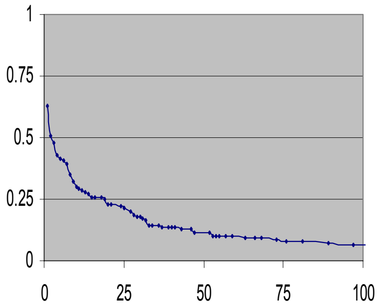
Figure 3: Graph of root mean squared deviation vs. total event size for a weakly linked model ( \varepsilon=0.1 ).
