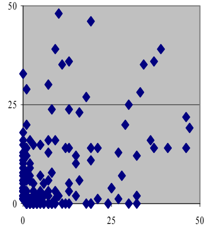
(b) \epsilon=0.1
