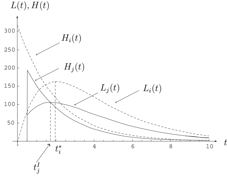
Figure 1: Overall profit functions for \gamma = 0.5
