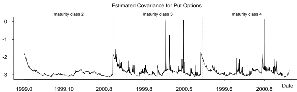
Figure 1: Covariance Between Residuals in the Regression and the Selection Equation
