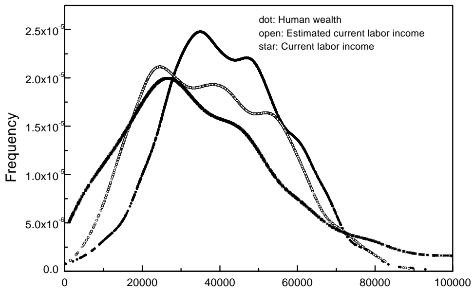
Figure1: Kernel Density Estimation
