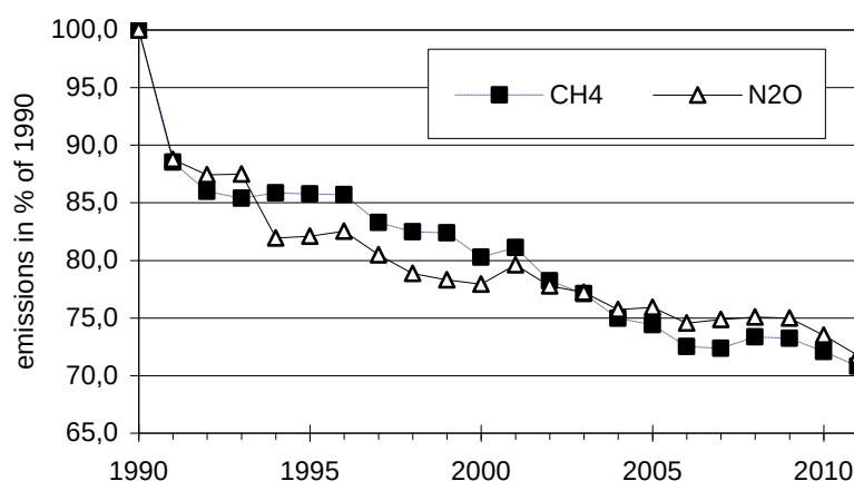
Figure 2.2: Development of CH 4 and N 2 O emissions from manure management in % of 1990, Submission 2013
