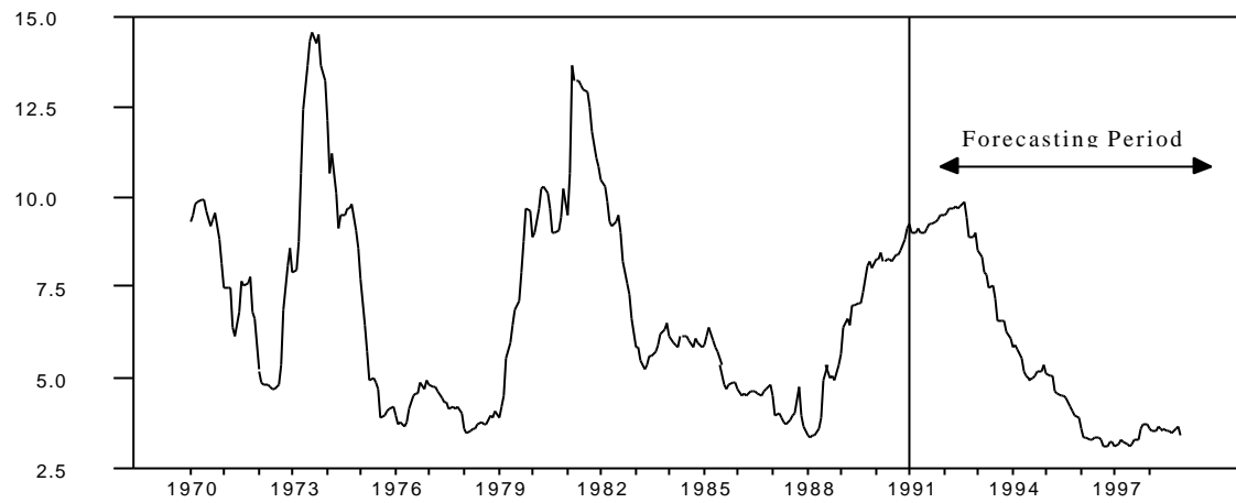
Figure 1: Short-term interest rate 1970-1998
