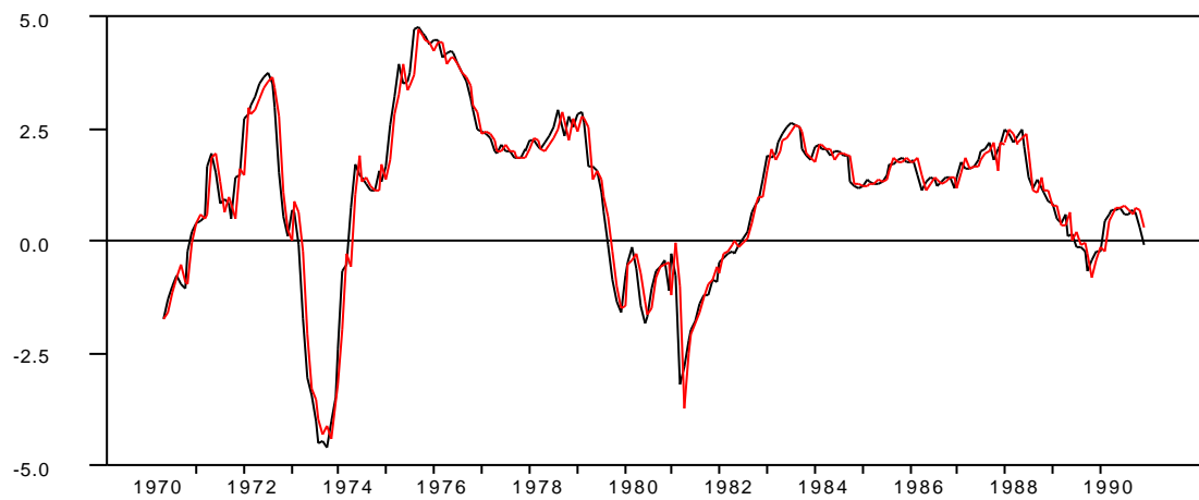
Figure 6: Contribution of the Markov chain to the spread RSH-VAR(1) model for differenced short rate and spread
