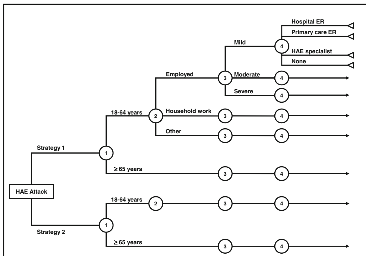
Figure 1 Simplified model of decision tree. Icatibant administration: Strategy 1= Health professional-administration only; Strategy 2= Self-administration also available. HAE: Hereditary angioedema. ER: Emergency room.
