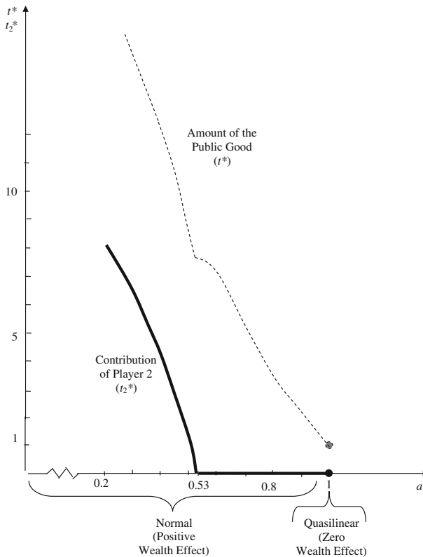
Fig. 2 The equilibrium correspondence as the wealth effect tends to zero: Example 2: Two players with different preferences
