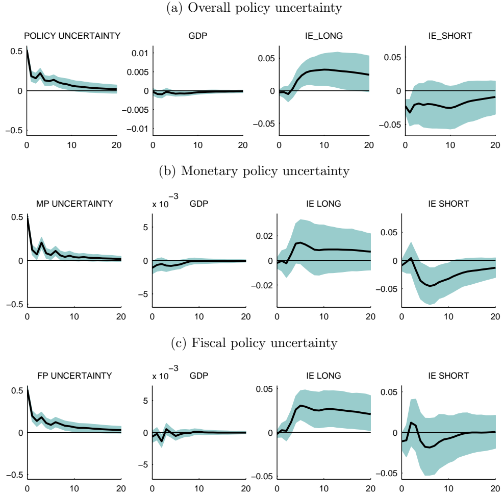
Figure 12: IRFs to a policy uncertainty shock for Germany
