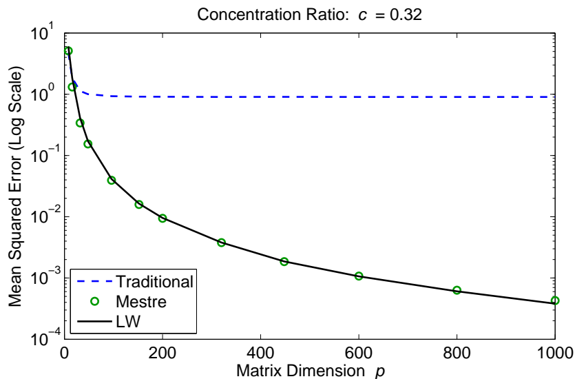
Figure 4: Convergence of estimated eigenvalues to population eigenvalues when eigenvalues are grouped into a small number of high-multiplicity clusters.
