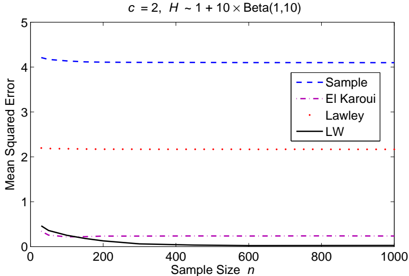
Figure 2: Convergence of estimated eigenvalues to population eigenvalues in the case where the sample covariance matrix is singular.
