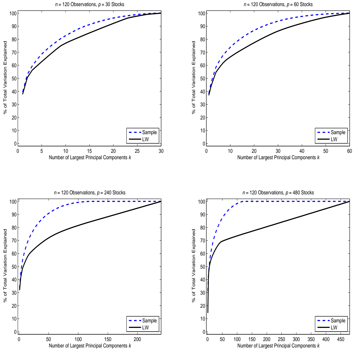
Figure 7: Percentage of total variation explained by the k largest principal components of stock returns: estimates based on the sample covariance matrix (Sample) compared to those based on nonlinear shrinkage (LW).
