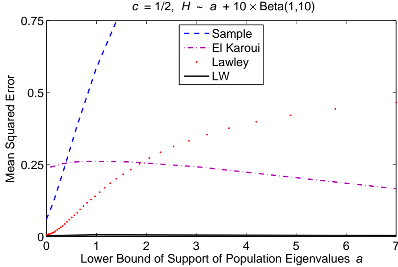
Figure 3: Effect of the condition number on the mean squared error between estimated and population eigenvalues.
