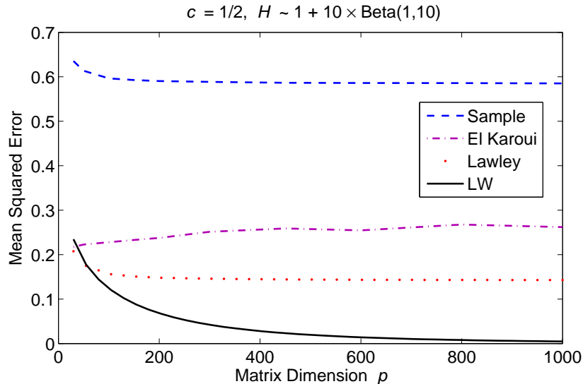
Figure 1: Convergence of estimated eigenvalues to population eigenvalues in the case where the sample covariance matrix is nonsingular.
