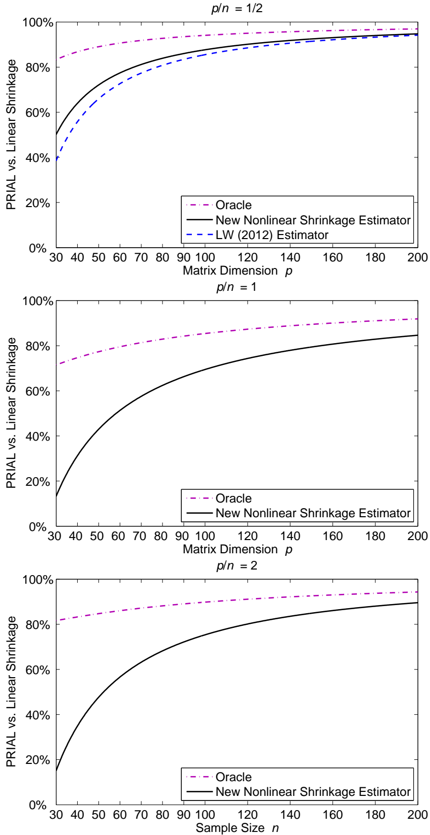
Figure 5: Percentage Improvement in Average Loss (PRIAL) according to the Frobenius norm of nonlinear versus linear shrinkage estimation of the covariance matrix.
