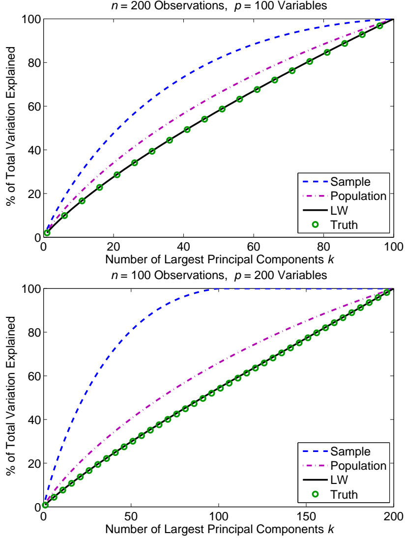
Figure 6: Comparison between different estimators of the percentage of total variation explained by the top principal components.
