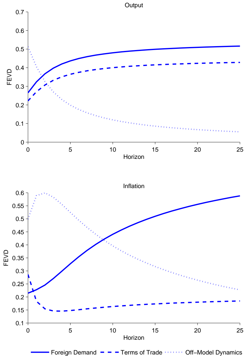
Figure 7: Forecast Error Variance Decomposition
