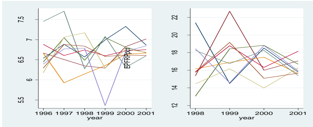
Figure A1: Time-series plot of log yield against year and EPFRPpct against year for ages 20-30
