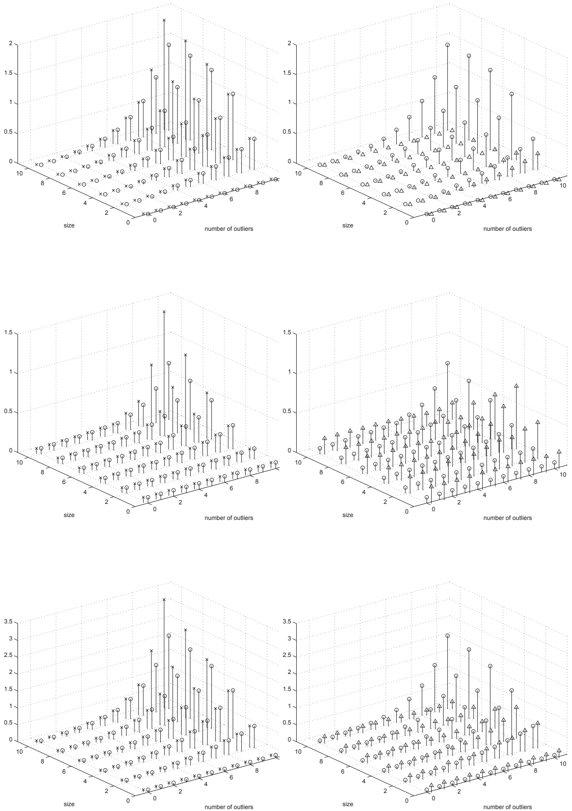
Figure 2: Steady state: Simulated squared bias (top), variance (middle) and MSE (bottom) for the intercept. L_1 regression \times , repeated median \circ and LMS \Delta .
