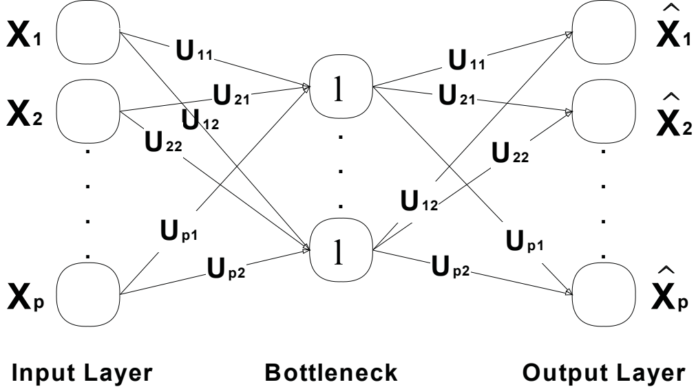
Figure 2: Neural network for principal component analysis.
