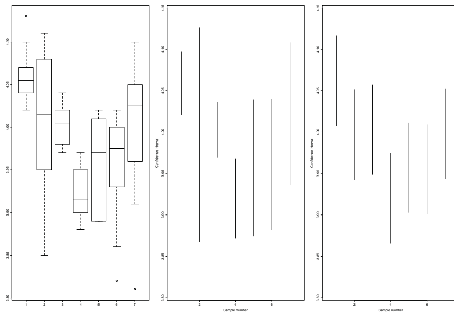
Figure 1: Box-plots and approximation intervals for the data from Rice (1988). Second panel shows intervals based on the default functionals with local scales, the third panel shows intervals based on the mean and a global standard deviation.
