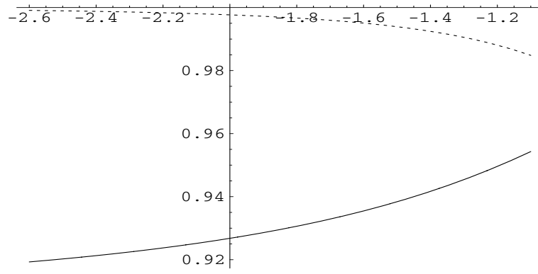
Figure 4.1: Efficiencies of the E -optimal design \xi^*(b) for estimating the individual coefficients in the regression model (4.9) for various values of b \in [-2.5, -1] . Solid line: \text{eff}_1(\xi^*(b)) , dotted line: \text{eff}_2(\xi^*(b)) .
