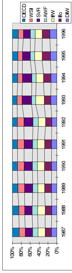
Squared ranks
