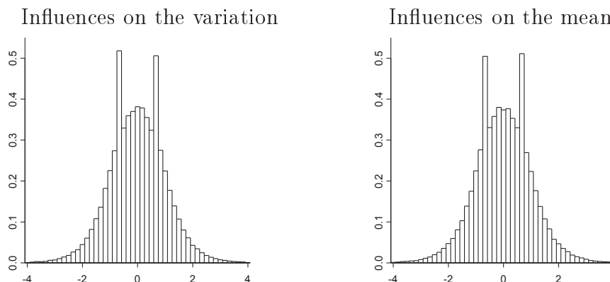
Figure 11: Empirical Distribution of Standardized Effects, t -values computed by using the Median-based variance estimator, \lambda set to 1
