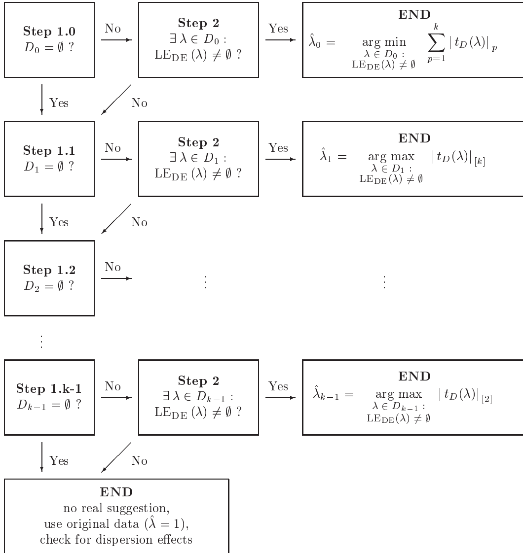
Figure A.1: Flow-chart for the Formalized \lambda -Plot procedure
