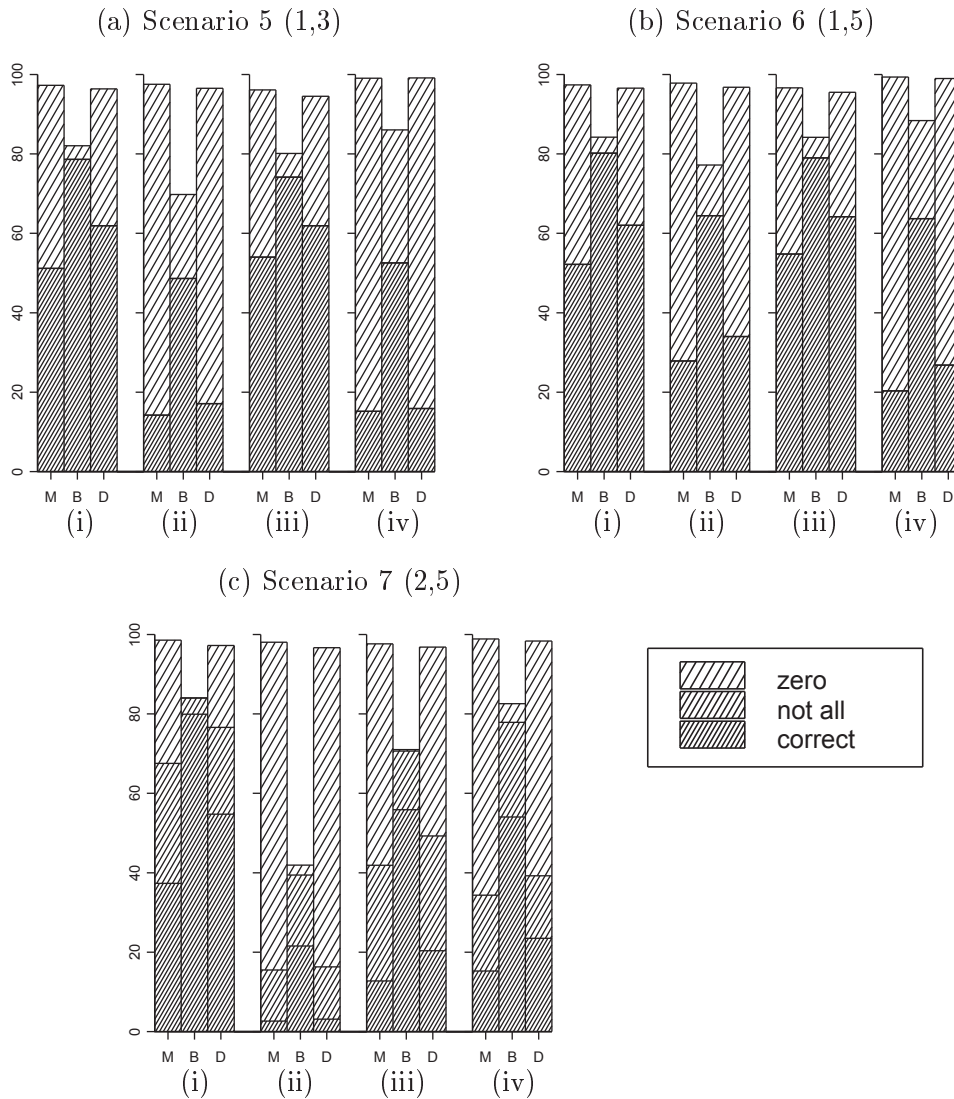
Figure 9: Identified effects on the variation, (i) \lambda = 1 (reference); (ii) \hat{\lambda} from Original \beta -Method; (iii) \hat{\lambda} from \beta -Method with s = 1 ; (iv) \hat{\lambda} from \lambda -Plot
