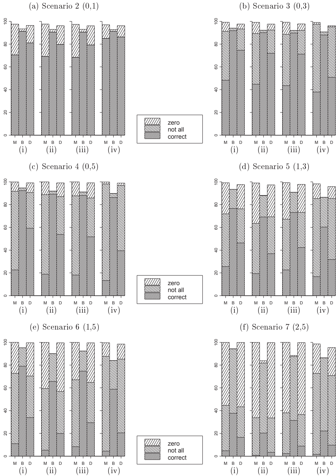
Figure 10: Identified effects on the mean, (i) \lambda = 1 (reference) (ii) \hat{\lambda} from Original \beta -Method (iii) \hat{\lambda} from \beta -Method with s = 1 (iv) \hat{\lambda} from \lambda -Plot
