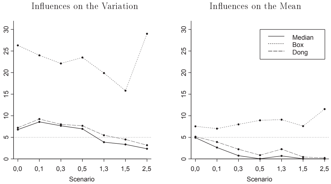
Figure 7: Percentage of data sets with wrongly identified effects, transformation parameter \lambda estimated by \beta -Method assuming one dispersion effect ( s=1 ), depending on the variance estimation method
