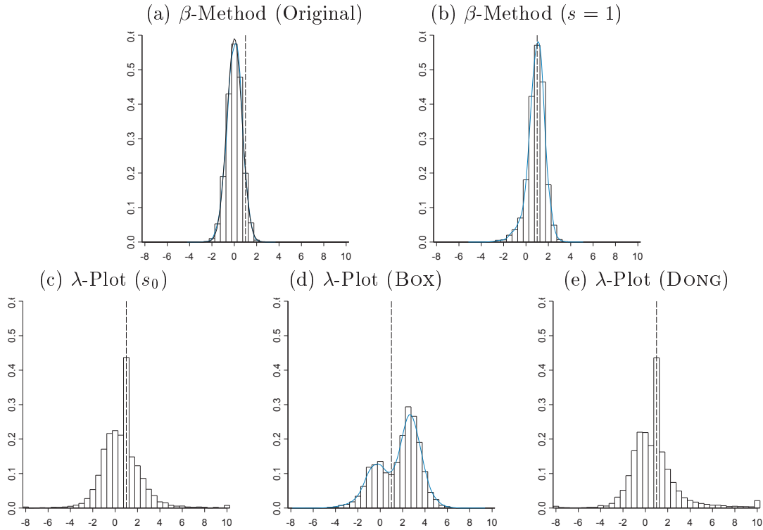
Figure B.3: Estimated \lambda -values for data sets containing one dispersion effect and four additional adjustment effects (Scenario 6)
