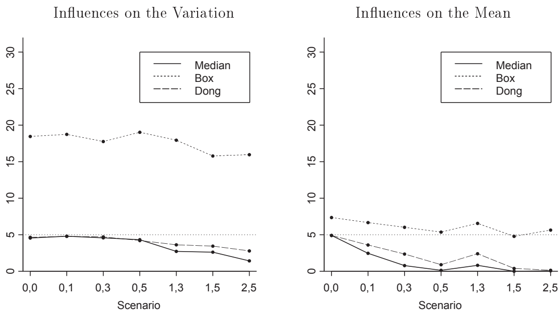
Figure 5: Percentage of data sets with wrongly identified effects for the true transformation parameter \lambda^* = 1 , depending on the variance estimation method
