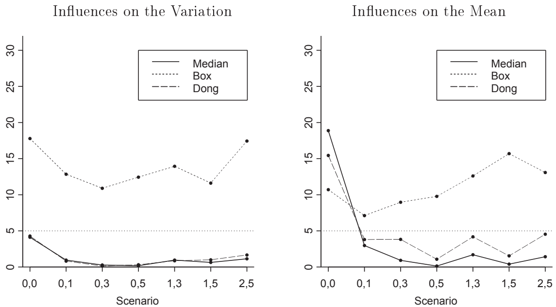
Figure 8: Percentage of data sets with wrongly identified effects, transformation parameter \lambda estimated by \lambda -Plot, depending on the variance estimation method
