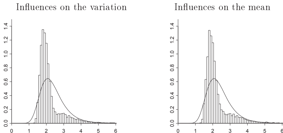
Figure 13: Empirical Distribution of Standardized Effects, t -values computed with variance estimator proposed by DONG, \lambda set to 1
