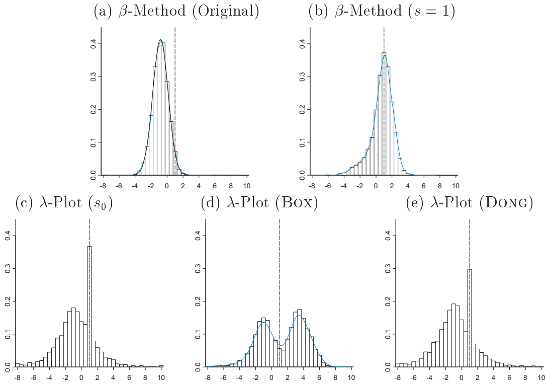
Figure 3: Estimated \lambda -values for data sets containing one dispersion effect and two additional adjustment effects (Scenario 5)
