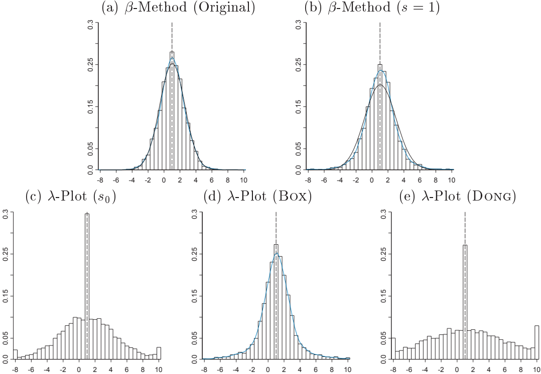
Figure B.2: Estimated \lambda -values for data sets containing five location effects (Scenario 4)
