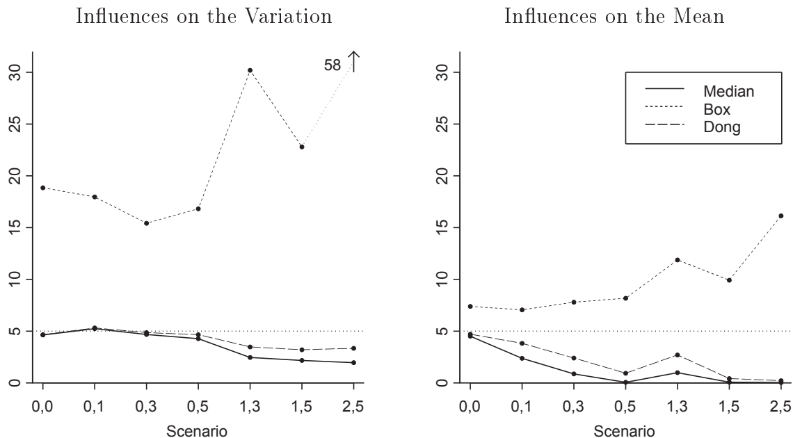
Figure 6: Percentage of data sets with wrongly identified effects, transformation parameter \lambda estimated by Original \beta -Method, depending on the variance estimation method
