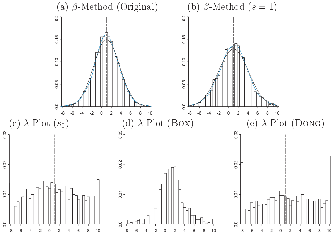
Figure 1: Estimated \lambda -values for data sets containing neither dispersion nor location effect (Scenario 1)
