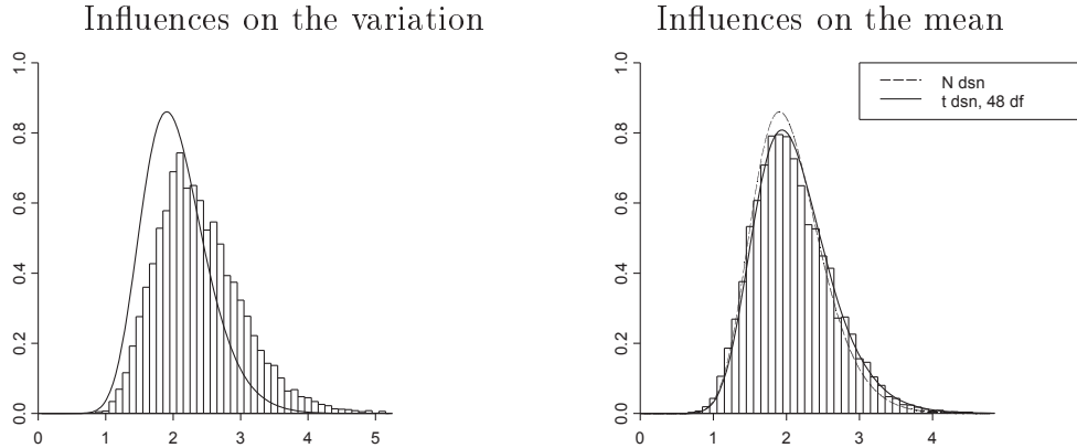
Figure 12: Empirical Distribution of unsigned maximum Standardized t -values, computed with variance estimators suggested by BOX, \lambda set to 1
