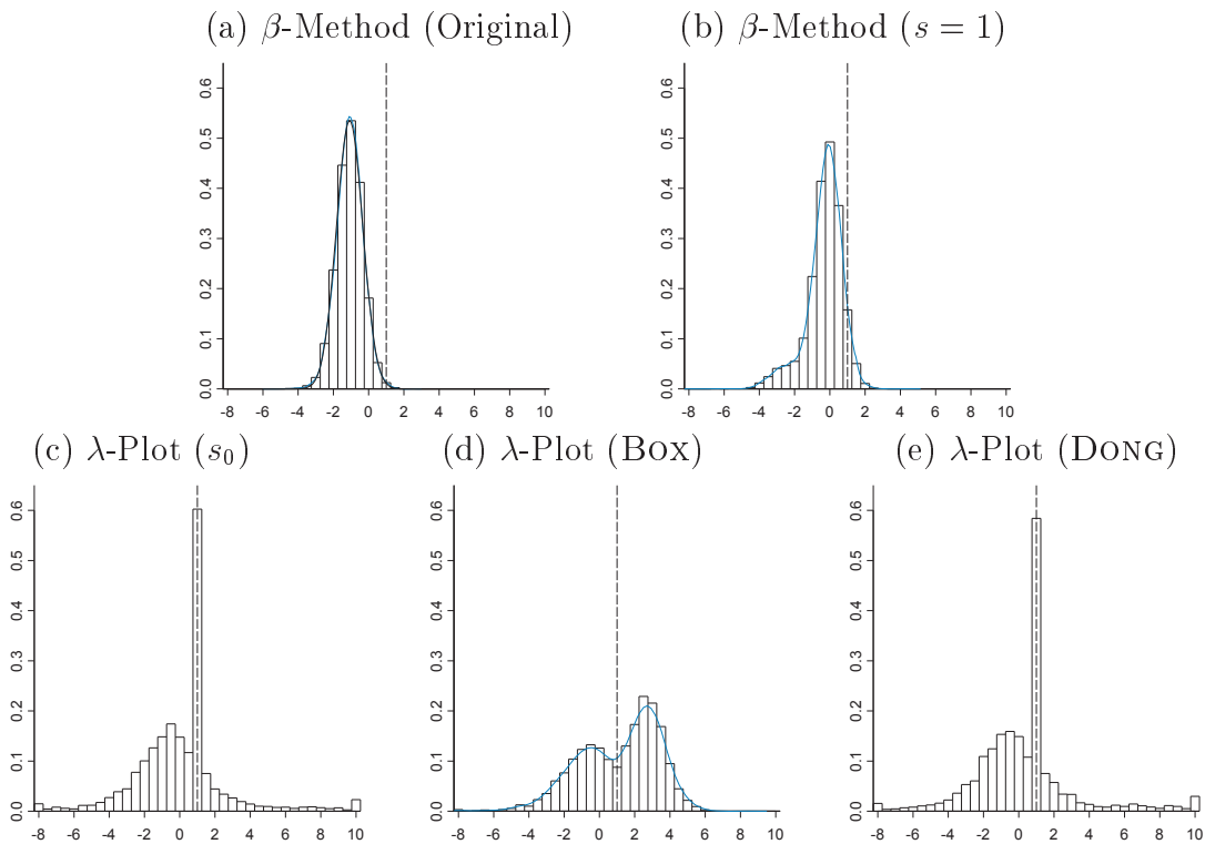
Figure 4: Estimated \lambda -values for data sets containing two dispersion effects and three additional adjustment effects (Scenario 7)
