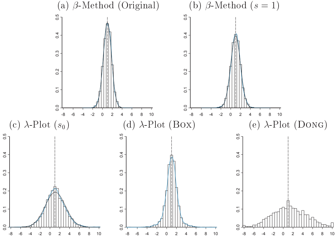
Figure 2: Estimated \lambda -values for data sets containing three location effects (Scenario 3)
