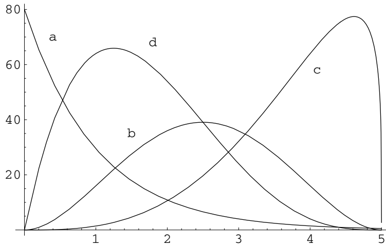
Figure 1: Different shapes of the efficiency functions on [0, 5] ; (a) \lambda_2(x, \theta) with (\theta_1, \theta_2)^T = (80, 1) and \lambda_3(x, \theta) with (b) (\theta_1, \theta_2)^T = (2, 2) , (c) (\theta_1, \theta_2)^T = (3, 0.25) and (d) (\theta_1, \theta_2)^T = (1, 3) .
