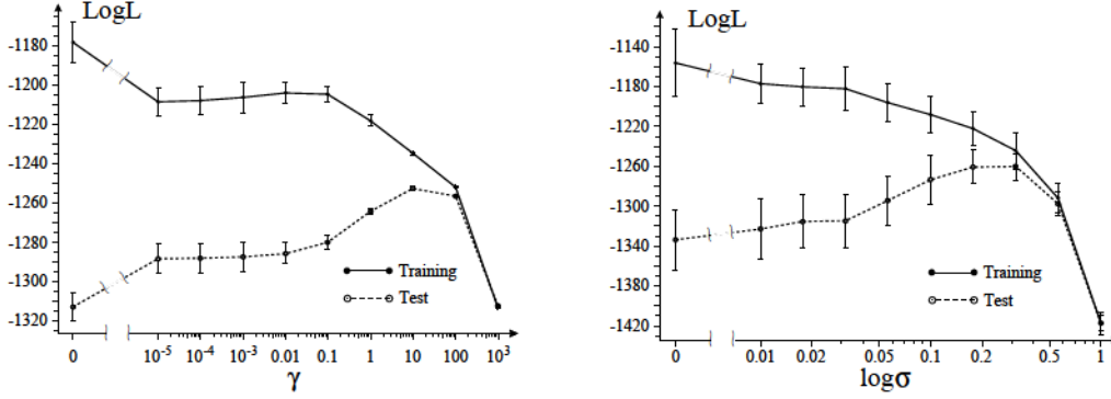
Figure 5: (left) Regularization with a roughness penalty, (right) regularization with noisy training samples. In both cases the log-likelihood of the training sample (solid line) and the test sample (dashed line) is shown for different values of the respective regularization parameter. All results are averaged over 100 runs.
