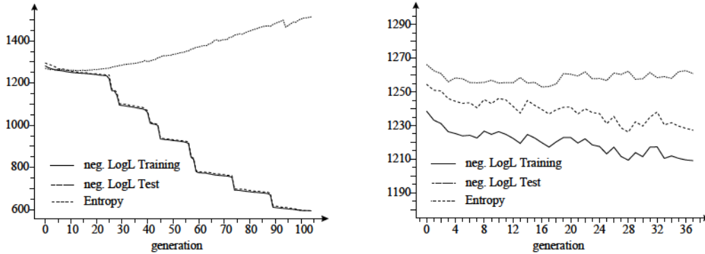
Figure 6: (left) Evolution of a Gaussian mixture without any regularization, (right) using the information criterion. The solid line shows the log-likelihood of the training sample and the dotted line the log-likelihood of the test sample, respectively. For comparison the entropy is shown by the dashed line.
