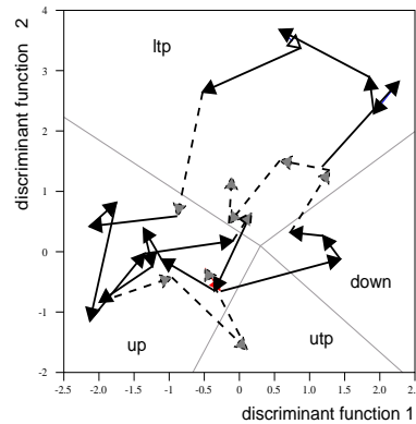
Figure 1: Linear Discriminant Analysis - one region per class
