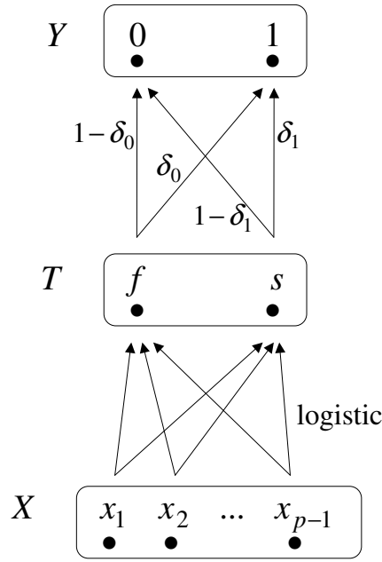
Fig. 2. Hidden logistic regression model.
